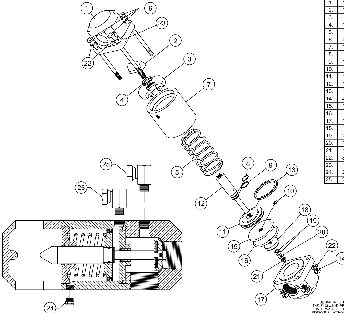
SECTION VIEW
